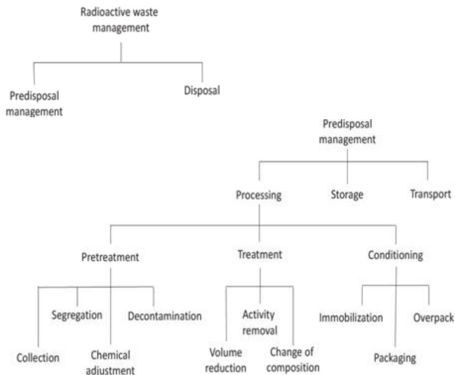
Figure 1: Steps of radioactive waste management, based on IAEA (2006)
